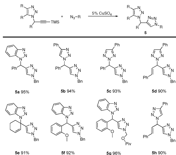
Figure 2. Synthesis of unsymmetrical N–C type bis-triazoles. Isolated yields for all cases. Condition: 0.05 equiv of CuSO 4 , 0.1 equiv of sodium ascorbate, t -BuOH-H 2 O (1:1), rt, 12 h. Structure 5g was confirmed by X-ray crystallography.
