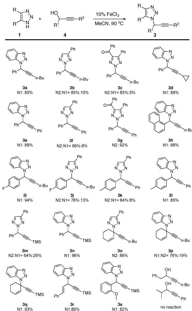
Figure 1. Reaction substrate scope. Yields were determined by NMR with 1,3,5-trimethoxybenzene as internal standard, and ratios determined by NMR of crude reaction mixtures. The N-2 3f structure was confirmed by X-ray crystallography.
