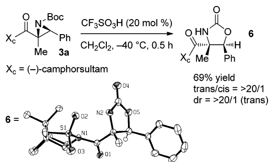
Scheme 3. Acid-Catalyzed Ring Rearrangement of Aziridine to Oxazolidin-2-one
