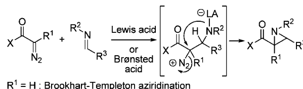
Figure 1. Acid-catalyzed aziridination of \alpha -diazocarbonyl compounds and imines.
