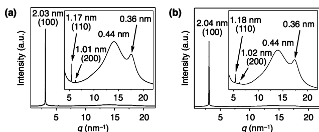
Figure 2. XRD patterns of bulk samples of (a) TP 8 containing 10 wt% of poly- 1 and (b) TP 8 containing 10 wt% of 1 at 70 °C on cooling from their isotropic melts. The samples were placed in a glass capillary ( \varphi = 1.5 mm). Values in parentheses indicate Miller indices. Insets show magnified XRD patterns in a wide-angle region. Based on the hkl = 100 diffraction peaks, lattice parameters were determined as 2.34 and 2.35 nm for poly- 1 -containing TP 8 (10 wt%) and 1 -containing TP 8 (10 wt %), respectively.
