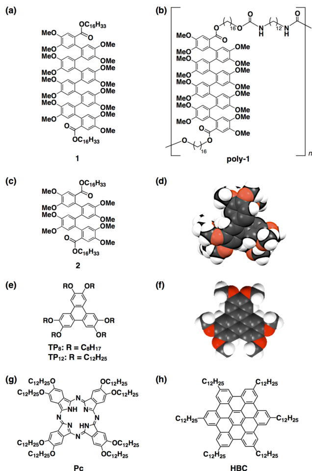
Figure 1. Molecular structures of (a) monomeric ( 1 ) and (b) polymeric (poly- 1 ) o -phenylene octamers and (c) o -phenylene tetramer ( 2 ). Molecular structures of discotic LC molecules derived from (e) triphenylene ( TP 8 and TP 12 ), (g) phthalocyanine ( Pc ), and (h) hexabenzocoronene ( HBC ). CPK models of (d) a hydrogen-terminated octamer of 1,2-dimethoxybenzene and (f) hexamethoxytriphenylene.
