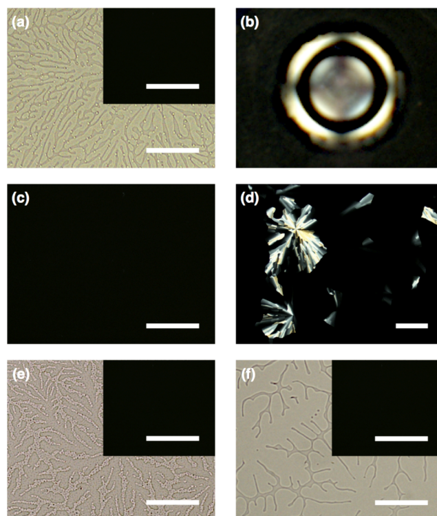
Figure 3. (a) OM and POM (inset) and (b) conoscopic image of a LC film of TP 8 containing 10 wt% of poly- 1 . (c) POM of a LC film of TP 8 containing 3 wt% of poly- 1 . (d) POM of a LC film of TP 8 alone. (e) OM and POM (inset) of a LC film of TP 8 containing 10 wt% of 1 . (f) OM and POM (inset) of TP 8 on a glass substrate spin-coated with poly- 1 . All LC samples were heated once to their isotropic melting point, allowed to cool to 70 °C, and then subjected to microscopy. Scale bars for (a) and (c)–(e) represent 100 \mu m, and that for (f) denotes 50 \mu m.
