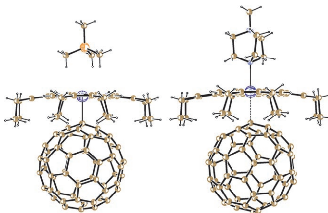
Figure 1. Molecular structures of the \sigma -bonded \{\text{Co}^{\text{II}}\text{OEP}(\text{C}_{60}^-)\} unit in 1 (left) and the \{(\text{MDABCO}^+)(\text{Co}^{\text{II}}\text{OEP}(\text{C}_{60}^-))\} assembly in 2 (right). Only the major orientation for disordered \text{C}_{60}^- is shown for 1 and 2 and one orientation of disordered \text{MDABCO}^+ is shown for 2 .
