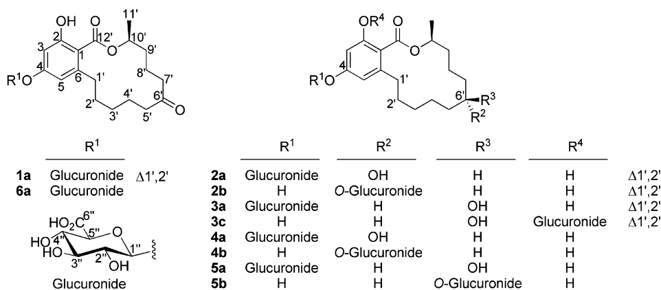
Figure 3. Structures of glucuronide derivatives of zearalenone metabolites 1 – 6 isolated in this study after enzymatic synthesis. In the text, glucuronides of compounds 1 – 6 with glucuronic acid attached via C-4 are designated a (e.g., 1a is zearalenone 4- O - \beta -D-glucuronide), whereas compounds with glucuronic acid attached via C-6' are designated b (e.g., 2b is \alpha -zearalenol 6'- O - \beta -D-glucuronide) and compounds with glucuronic acid conjugated via C-2 are designated c (e.g., 3c is \beta -zearalenol 2- O - \beta -D-glucuronide).
