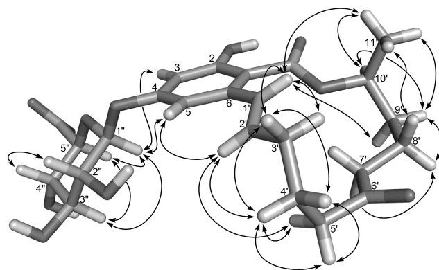
Figure 6. Calculated structure of zearalenone 4- O - \beta -D-glucuronide ( 1a ) sodium salt, showing selected correlations observed in the NOESY NMR spectrum in \text{CD}_3\text{OD} .
