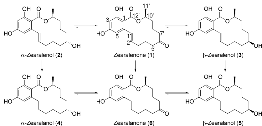
Figure 1. Structures of resorcylic acid lactones and the proposed metabolism of zearalenone in cattle and sheep (7). Double arrows indicate readily reversible oxidation/reduction of the oxygen atom at C-6'.
