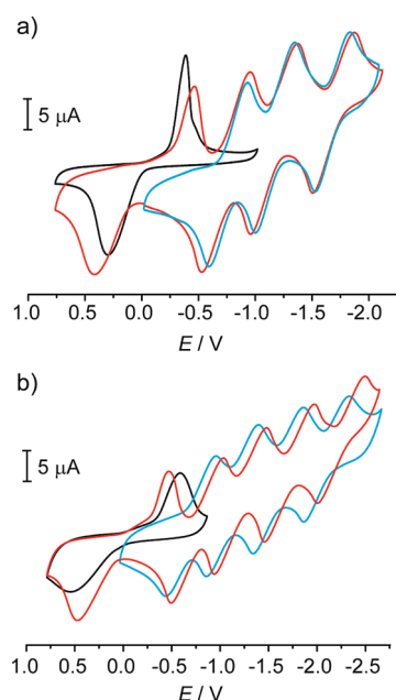
Figure 8. Cyclovoltammograms of (a) p -xylnac12 (black), C_{60} (blue), and p -xylnac12· C_{60} (red); (b) naphmac14 (black), C_{70} (blue), and naphmac14· C_{70} (red), in PhCl, Bu_4NClO_4 (0.1 M), \nu = 0.1 \text{ V s}^{-1} , [fullerene] = [macrocycle] = 5 \times 10^{-4} \text{ M} . Potentials are indicated vs the Ag/AgNO 3 redox couple.
