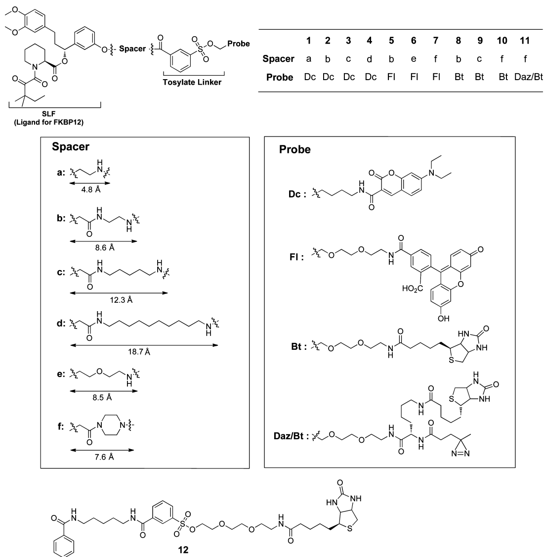
Figure 2. Molecular structures of LDT reagents for FKBP12 (1–11) and control compound 12 . SLF, synthetic ligand of FKBP12; Dc, 7-diethylaminocoumarin; Fl, 5-carboxyfluorescein; Bt, biotin; Daz, diazirine.
