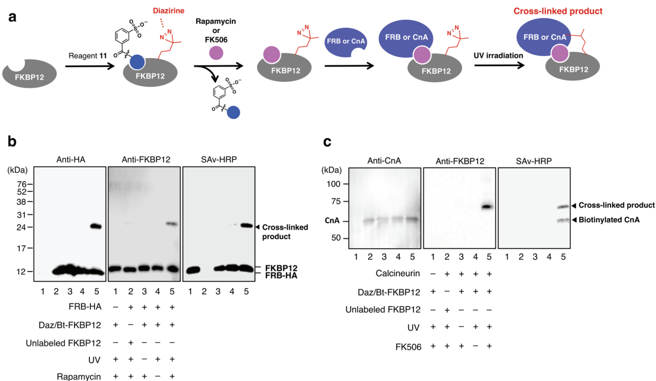
Figure 7. In vitro photo-cross-linking. (a) Schematic illustration of the strategy. (b) Western blotting analysis of photo-cross-linking of Daz/Bt-FKBP12 with FRB-HA. Reaction conditions: 1 \mu M Daz/Bt-FKBP12 (postlabeling solution) or unlabeled FKBP12, 3 \mu M FRB-HA, 5 \mu M rapamycin, UV light (365 nm, 20 min), 50 mM Tris buffer, pH 8.0, on ice. (c) Western blotting analysis of photo-cross-linking of Daz/Bt-FKBP12 with CnA. Reaction conditions: 0.1 \mu M Daz/Bt-FKBP12 (postlabeling solution) or unlabeled FKBP12, 0.3 \mu M Cn, 1 \mu M FK506, UV light (365 nm, 20 min), 50 mM Tris buffer, pH 8.0, on ice.
