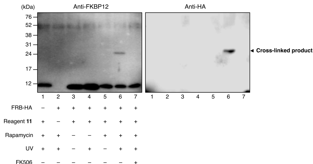
Figure 8. Photo-cross-linking of endogenous FKBP12 with its interacting protein (FRB-HA) in live cells. After HeLa cells transiently expressing FRB-HA were incubated with 11 ( 5\ \mu\text{M} ) for 18 h, the cells were UV irradiated (20 min) in the absence or presence of rapamycin ( 5\ \mu\text{M} ) and lysed. All biotinylated proteins were captured and purified with NeutrAvidin beads and subjected to Western blotting analysis.
