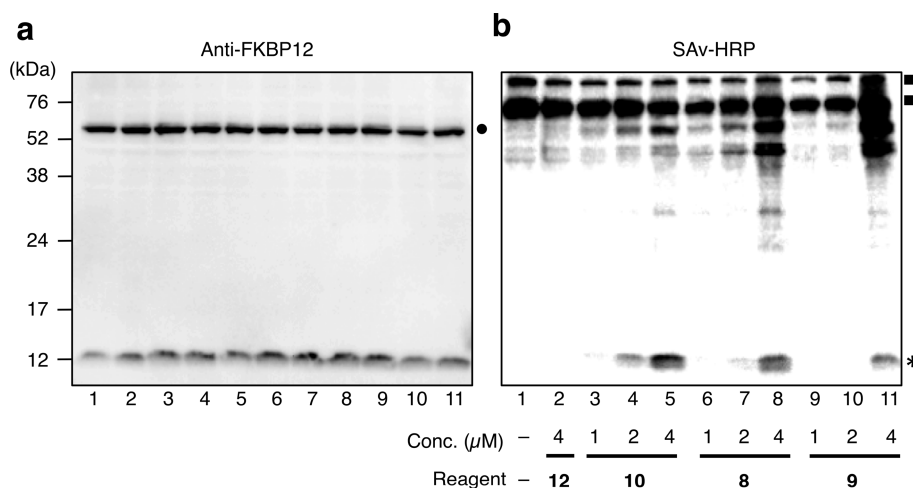
Figure 6. Chemical biotinylation of FKBP12 in Jurkat cells using 8 – 10 and 12 . Reaction conditions: Jurkat cells ( 4 \times 10^6 cells), 1–4 \mu M LDT reagent, serum-free RPMI 1640 medium, 37 ^{\circ} C, and 18 h. After labeling, the cells were washed, lysed, and analyzed by Western blotting. (a) Detection by anti-FKBP12 antibody; ●, nonspecific band. (b) Detection by SAV-HRP; ■, endogenous biotinylated protein; *, Bt-labeled FKBP12.
