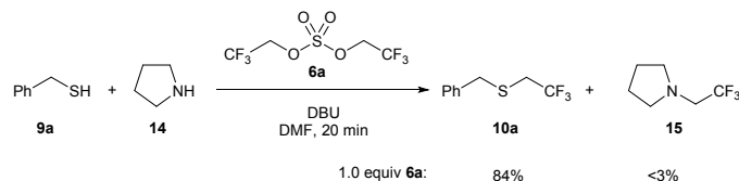
Scheme 5 Competition experiments with sulfur and nitrogen nucleophiles.
