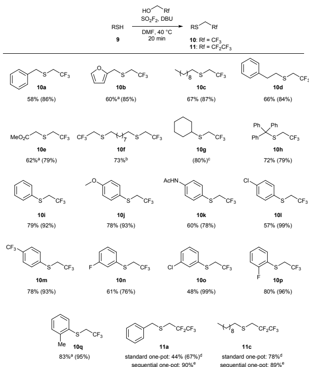
Scheme 3 Substrate scope for the 1,1-dihydrofluoroalkylation of thiols. Reaction conditions: SO 2 F 2 (2.9 equiv) was bubbled through a solution of 9 (1 equiv), DBU (5.9 equiv) in 1:1 TFE/DMF (v/v), at 40 °C for 3 minutes, and then the reaction was stirred for an additional 17 min. All reactions were run on 1 mmol scale of thiol unless otherwise indicated. Isolated yields for the one-pot reaction are reported, with 19 F NMR yields (using trifluorotoluene as the internal standard) provided in parentheses. a The isolated yield has been corrected to account for disulfide or solvent impurities. See the Supplementary Information for details. b The reaction was conducted on 0.5 mmol scale. c The product was not isolated due to volatility. d The reaction was stirred for 2 hours. e Pentafluoropropanol:DMF (1:2 v/v) was used to form the reagent, and then the thiol was added to the reaction mixture. The reaction was stirred for 30 minutes.
