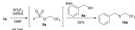
Scheme 2 Investigations into thiol alkylation using fluorosulfate ( 5a ) and bis(trifluoroethyl) sulfate ( 6a ). The yields in B and C were determined by 19 F NMR spectroscopy using trifluorotoluene as an internal standard.
