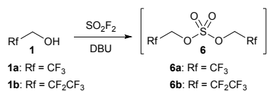
Scheme 1 Representative examples of sulfuranyl fluoride-mediated processes that utilize fluorosulfate reactive intermediates ( 5 ) and a new bis(trifluoroalkyl) sulfate ( 6 ).
