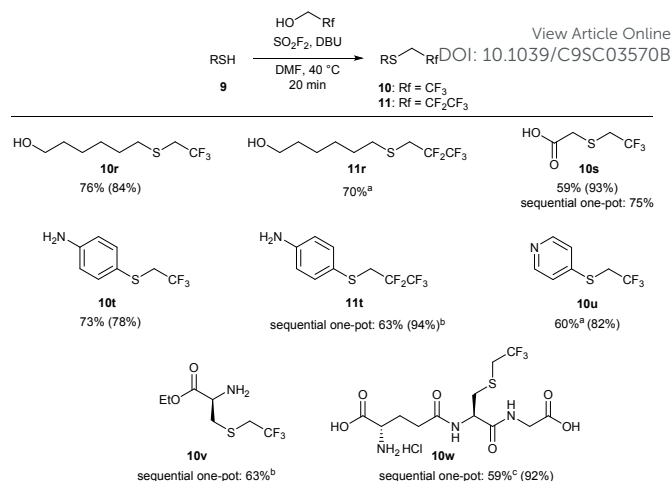
Scheme 4 Functional group tolerance of the 1,1-dihydrofluoroalkylation reaction. Reaction conditions: SO 2 F 2 (2.9 equiv) was bubbled through a solution of 9 (1 equiv), DBU (5.9 equiv) in 1:1 TFE/DMF (v/v), at 40 °C for 3 minutes, and then the reaction was stirred for an additional 17 min. All reactions were run on a 1 mmol scale unless otherwise indicated. Isolated yields for the one-pot reaction are reported, with 19 F NMR yields (using trifluorotoluene as the internal standard) provided in parentheses. a The one-pot reaction was stirred for 2 hours. b The sequential, one-pot reaction was stirred for 30 minutes after addition of thiol. c The product was converted to an HCl salt, and the reported yield has been corrected for solvent impurities.
