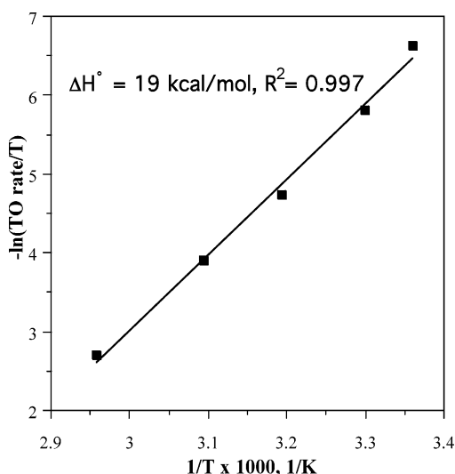
Figure 4. Eyring plot for adamantane hydroxylation with 2,6-dichloropyridine N -oxide catalyzed by Ru VI (TPFPP)(O) 2 . [adamantane] = 0.02 M, [Ru VI (TPFPP)(O) 2 ] = 50 \mu M, [2,6-dichloropyridine N -oxide] = 0.02 M; CH 2 Cl 2 ; 40 °C.
