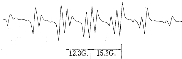
Fig. 1. The ESR Spectrum of \text{Me}_2\text{N}\dot{\text{O}} obtained during the Controlled Potential Electrolysis of \text{Me}_2\text{NOH}
