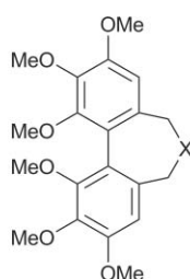
66 X = NBn 67 X = NMe 68 X = S 69 X = SO 70 X = SO 2
