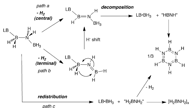
Scheme 5. Possible Dehydrogenation Reaction Pathways for H 2 BNH 2 Adducts
