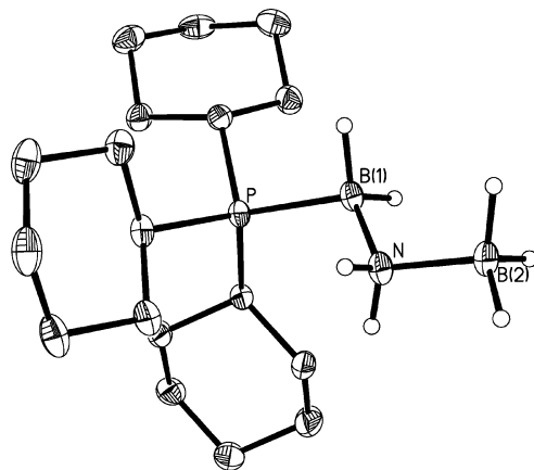
Figure 1. Thermal ellipsoid plot (30% probability) of Cy 3 P–H 2 BNH 2 –BH 3 ( 3 ), with carbon-bound hydrogen atoms and dichloromethane solvate omitted for clarity. Compound 3 cocrystallized with 4% Cy 3 P–H 2 BNH 2 –BH 3 ·Cl. 19 Selected bond lengths [Å] and angles [deg]: P–B(1) 1.9730(17), B(1)–N 1.564(2), B(1)–H 1.155(18) and 1.086(18), N–H 0.847(19) and 0.93(2), N–B(2) 1.608(2), B(2)–H 1.164(18), 1.157(19), and 1.12(2); P–B(1)–N 115.61(11), B(1)–N–B(2) 114.84(13); P–B(1)–N–B(2) torsion angle = 174.29(12).
