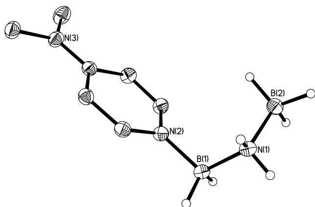
Figure 2. Thermal ellipsoid plot (30% probability) of \text{DMAP-H}_2\text{BNH}_2\text{-BH}_3 ( 4 ), with carbon-bound hydrogen atoms and hexane solvate molecules omitted for clarity. Selected bond lengths [Å] and angles [deg]: N(2)–B(1) 1.5728(15), B(1)–N(1) 1.5720(17), N(1)–B(2) 1.5939(16), B(1)–H 1.109(13), and 1.125(13), B(2)–H 1.102(15), 1.145(14) and 1.147(17); N(2)–B(1)–N(1) 110.44(9), B(1)–N(1)–B(2) 118.68(9); N(2)–B(1)–N(1)–B(2) torsion angle = 65.71(13).
