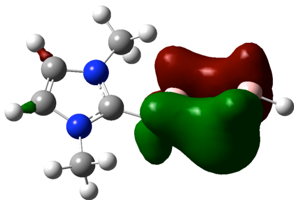
Figure 5. HOMO-18 for \text{ImMe}_2\text{CH}_2\cdot\text{H}_2\text{BNH}_2\cdot\text{BH}_3 ( 2' ) as derived from a DFT study showing orbital overlap between B–H and N–H bonding orbitals.
