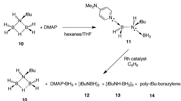
Scheme 6. Synthesis and Catalytic Dehydrogenation of DMAP·H 2 BNH( t Bu)-BH 3 ( 11 )
