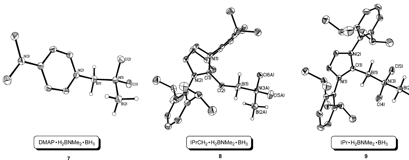
Figure 4. Thermal ellipsoid plots (30% probability) of DMAP- \text{H}_2\text{BNMe}_2\cdot\text{BH}_3 ( 7 ), \text{IPrCH}_2\cdot\text{H}_2\text{BNMe}_2\cdot\text{BH}_3 ( 8 ), and \text{IPr}\cdot\text{H}_2\text{BNMe}_2\cdot\text{BH}_3 ( 9 ) with carbon-bound hydrogen atoms and solvate molecules omitted for clarity; compound 8 contains a disordered \text{NMe}_2\text{BH}_3 unit. Selected bond lengths [Å] and angles [deg]: Compound 7 : N(2)–B(1) 1.5722(19), B(1)–N(1) 1.5801(18), N(1)–C(1) 1.4835(16), N(1)–C(2) 1.4800(17), N(1)–B(2) 1.6020(19), B(1)–H 1.115(14) and 1.104(15), B(2)–H 1.130(15), 1.130(16), and 1.126(18); N(2)–B(1)–N(1) 111.32(11), B(1)–N(1)–B(2) 114.53(11); N(2)–B(1)–N(1)–B(2) torsion angle = 60.99(15). Compound 8 ; values involving a disordered \text{NMe}_2\text{BH}_3 unit in square brackets: C(2)–B(1) 1.659(3), B(1)–N(3A) 1.589(6) [1.581(6)], N(3A)–C(5A) 1.507(13) [1.470(14)], N(3A)–C(6A) 1.496(12) [1.441(13)], N(3A)–B(2A) 1.596(14) [1.585(17)], C(2)–B(1)–N(3A) 106.2(4) [120.4(4)], B(1)–N(3A)–B(2A) 120.5(8) [106.9(9)]; C(2)–B(1)–N(3A)–B(2A) torsion angle = 52.9(7) [59.3(8)]. Compound 9 : C(1)–B(1) 1.639(2), B(1)–N(3) 1.588(2), N(3)–C(4) 1.477(2), N(3)–C(5) 1.475(2), N(3)–B(2) 1.617(2), B(1)–H 1.146(18) and 1.130(18), B(2)–H 1.12(2), 1.16(2), and 1.16(2); C(1)–B(1)–N(3) 114.39(12), B(1)–N(3)–B(2) 110.63(13); C(1)–B(1)–N(3)–B(2) torsion angle = 178.38(12).
