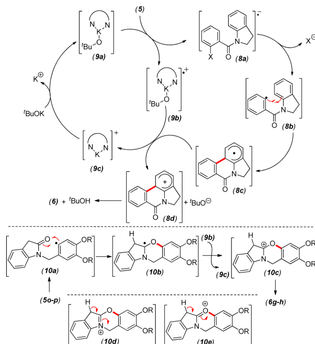
Figure 6. Proposed mechanism of intramolecular biaryl synthesis.
