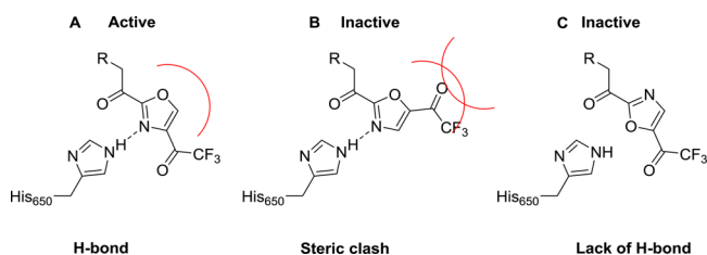
Figure 3. Proposed binding mode of substituted \alpha -keto oxazoles. (A) Meta ( X_4 ) substituted oxazole (exemplified by 45 ) forms a hydrogen bond with His650 and positions the substituent away from the highly sterically restricted pocket at X_5 . (B) Para ( X_5 ) substituted oxazoles (exemplified by 62 ) have a potential steric clash with the enzyme, possibly explaining their low potency on DAGL \alpha . (C) If the oxazole flips to avoid steric clash (para substituted), the oxazole nitrogen is excluded from hydrogen bond formation with His650.
