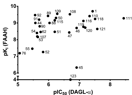
Figure 4. Graphical representation of DAGL \alpha inhibition ( pIC_{50} ) versus FAAH activity ( pK_i ). FAAH activity is that reported in the literature. 14,26–33 For a list with exact values, see Supporting Information .
