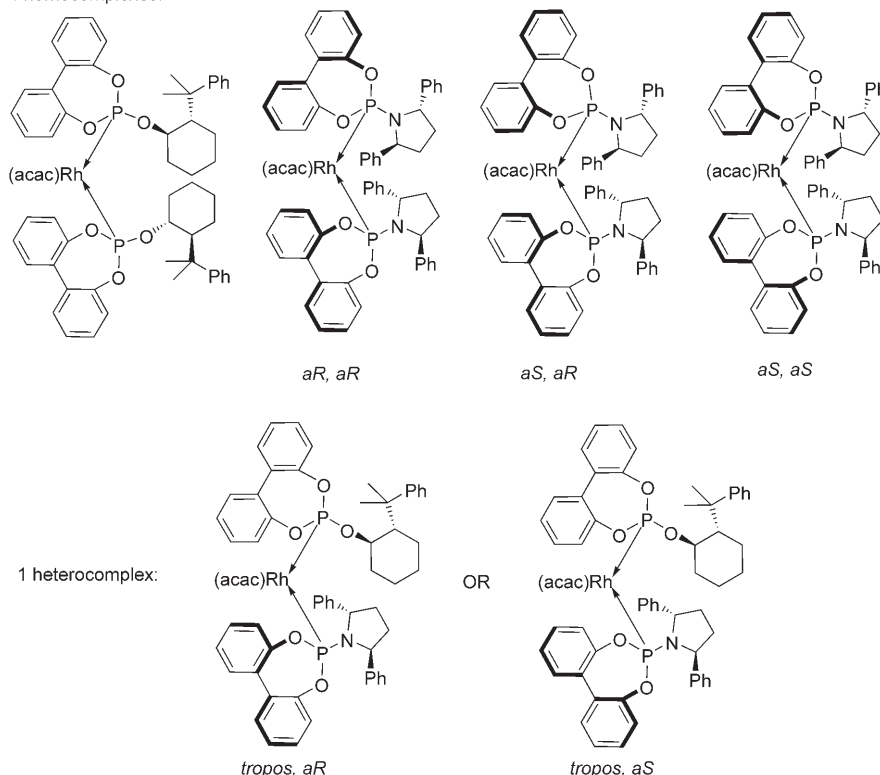
Scheme 4. The rhodium complexes ( [\text{Rh}(\text{acac})(\text{eth})_2] as the rhodium source) that originate from the combination of phosphite 6 -P(O) 2 O and phosphoramidite 19 -P(O) 2 N, at low temperature (230 K).
