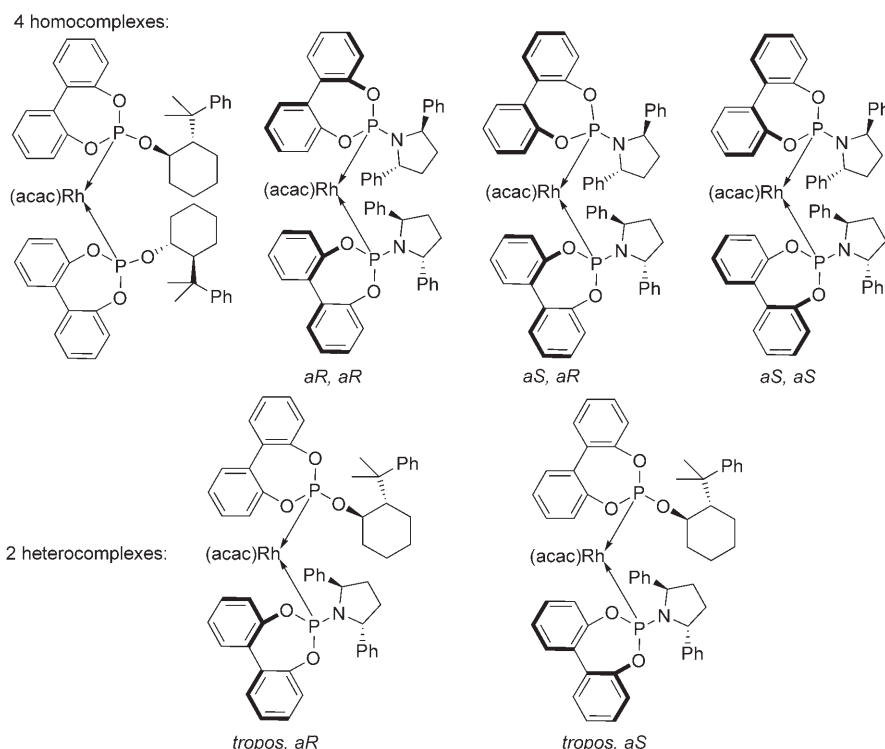
Scheme 5. The rhodium complexes ( [\text{Rh}(\text{acac})(\text{eth})_2] as the rhodium source) that originate from the mismatched combination of phosphite 6-P(O) 2 O and phosphoramidite 18-P(O) 2 N , at low temperature (230 K).
