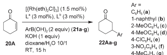
Scheme 2. Rh-catalyzed conjugate addition of arylboronic acids to 2-cyclohexenone ( 20A ).
