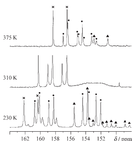
Figure 8. Variable-temperature ^{31}\text{P} NMR spectra ( [\text{D}_8]\text{toluene} ) of the rhodium complexes resulting from the combination of ligands 6\text{-P}(\text{O})_2\text{O} and 19\text{-P}(\text{O})_2\text{N} , with [\text{Rh}(\text{acac})(\text{eth})_2] as the rhodium source. At 375 K, [\text{Rh}\{6\text{-P}(\text{O})_2\text{O}\}_2] gives a doublet (x), [\text{Rh}\{19\text{-P}(\text{O})_2\text{N}\}_2] gives a doublet (A), and [\text{Rh}\{6\text{-P}(\text{O})_2\text{O}\}\{19\text{-P}(\text{O})_2\text{N}\}] gives two dds (●); at 230 K, [\text{Rh}\{19\text{-P}(\text{O})_2\text{N}\}_2] gives two dds (A) and a doublet (x), [\text{Rh}\{6\text{-P}(\text{O})_2\text{O}\}_2] gives a doublet (x), and [\text{Rh}\{(aR)\text{-}19\text{-P}(\text{O})_2\text{N}\}\{6\text{-P}(\text{O})_2\text{O}\}] gives two dds (●).
