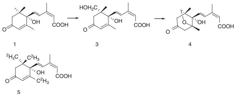
Scheme 1. Principal oxidative pathway of metabolism of ABA
