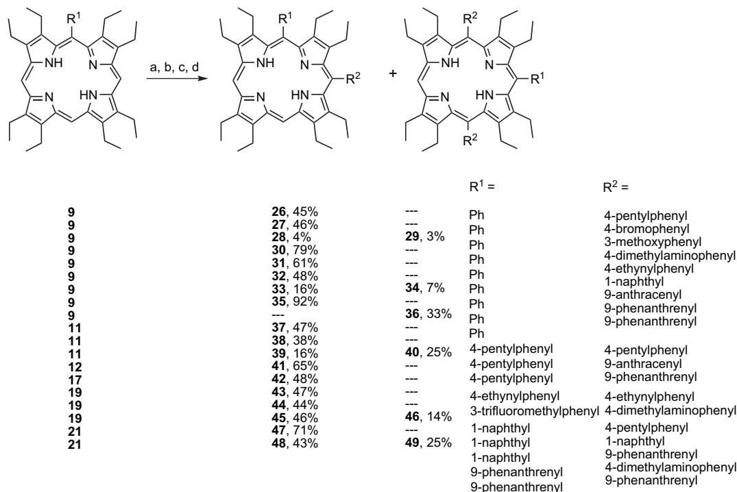
Scheme 2. Synthesis and yields of meso di- and trisubstituted 2,3,7,8,12,13,17,18-octaethylporphyrins. (a) LiR 2 , THF, –40 to –80 °C; (b) 1 h, rt; (c) H 2 O, 15 min; (d) DDO, 1 h.
