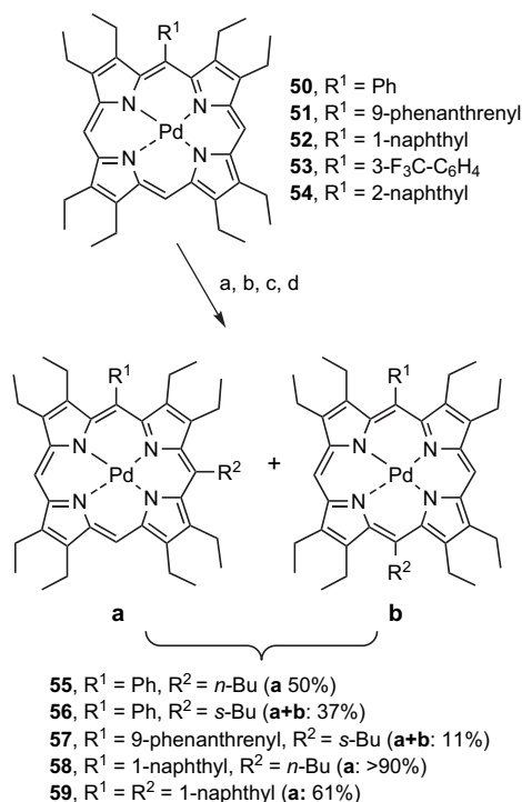
Scheme 3. Reactions of meso monosubstituted palladium porphyrins. (a) LiR 2 , THF, –40 to –80 °C; (b) 1 h, rt; (c) H 2 O, 15 min; (d) DDO, 1 h.
