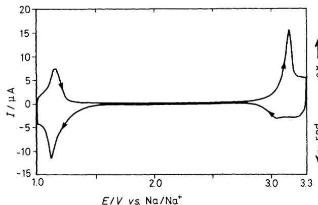
Figure 1. Cyclic voltammogram of a 5\text{ }\mu\text{m} poly(2,5-furylene vinylene) film versus a sodium counter and reference electrode in 1\text{ M NaPF}_6/\text{dimethoxyethane} . S = 0.1\text{ mV/s} .
