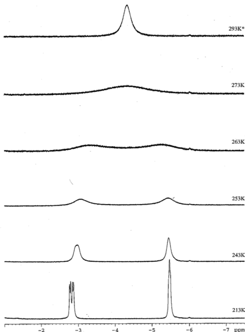
Figure 3. High field region of the ^1\text{H} NMR spectrum (toluene- d_8 , 400 MHz) of 4 at varying temperatures showing decoalescence at 273 K.
