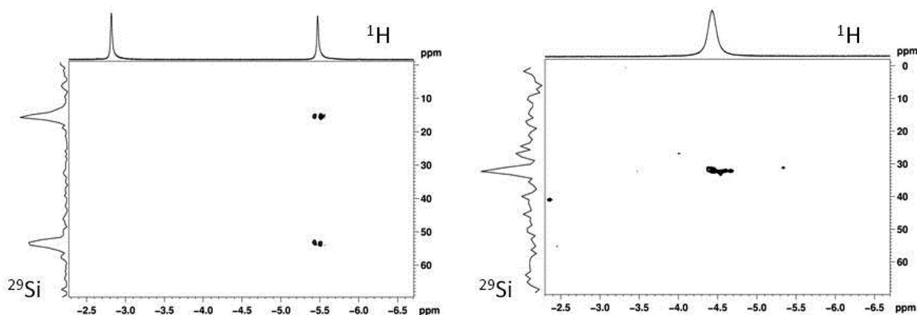
Figure 4. Region of the HMQC ^1\text{H} – ^{29}\text{Si}\{^{31}\text{P}\} NMR experiment at 324 K showing correlation of the silicon signal to the hydride resonance (H and H–Si), the two silicon, and the two hydrogen atoms around the ruthenium in complex 4 being in fast exchange (right). Region of the HMQC ^1\text{H} – ^{29}\text{Si}\{^{31}\text{P}\} NMR experiment at 213 K showing correlation of both silicon signals of 4 to only one high field ^1\text{H} resonance (H–Si) with the same J_{\text{Si-H}} of 37 Hz (left).
