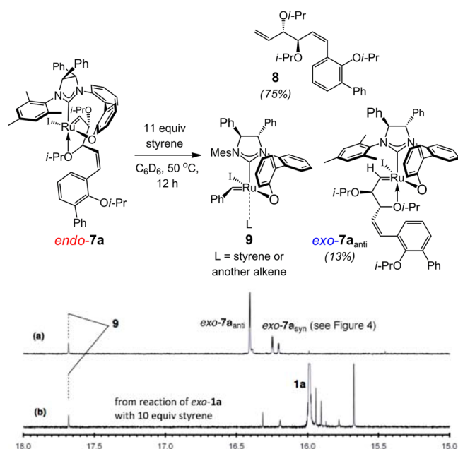
Figure 3. Reaction of endo - 7a with styrene, leading to exo carbenes 9 and exo - 7a anti , and 1 H NMR spectra (C 6 D 6 ) of (a) the reaction mixture prior to purification and (b) the mixture from treatment of pure 1a with 10 equiv of styrene (50 °C, 24 h). Percent values correspond to conversion determined by analysis of 400 MHz 1 H NMR analysis of the unpurified mixture; 8% conv to 7a syn and 4% conv to unidentified carbene. See the SI for details.
