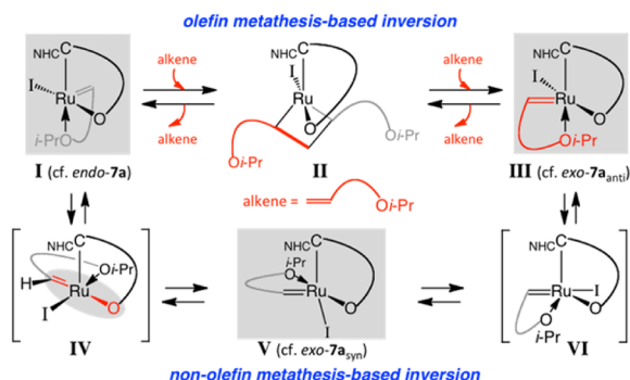
Scheme 2. Two Pathways for Stereochemical Inversion
