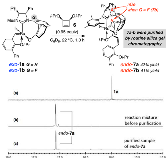
Figure 2. Syntheses of endo - 7a and endo - 7b by ROCM (yields are of pure products), and 1 H NMR spectra (C 6 D 6 ) of (a) pure 1a , (b) the mixture prior to purification, and (c) pure endo - 7a after silica gel chromatography. See the Supporting Information (SI) for details.
