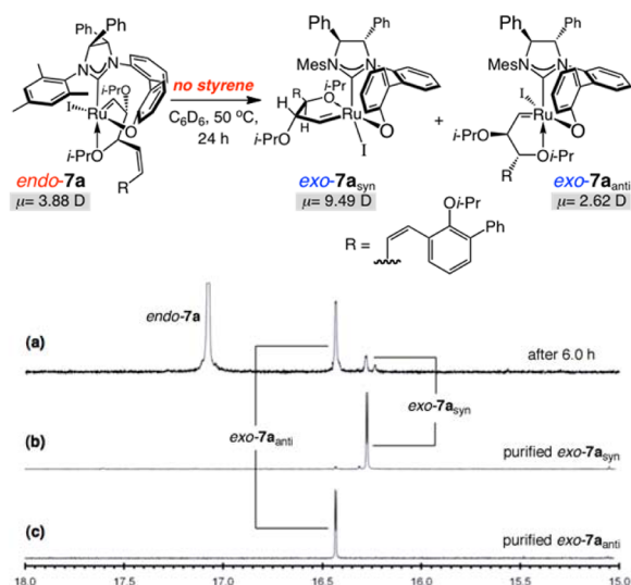
Figure 4. Thermal rearrangement of endo -7a, leading to exo -7a syn and exo -7a anti , and ^1H NMR spectra ( C_6D_6 ) of (a) the reaction mixture after 6.0 h, (b) isolated and purified exo -7a syn , and (c) isolated exo -7a anti . See the SI for details.
