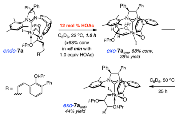
Scheme 3. Acid-Catalyzed Polytopal Rearrangement
