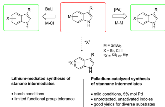
Scheme 1. Indirect Halogen–Radiohalogen Exchange at the Benzo Positions of Indole Derivatives
