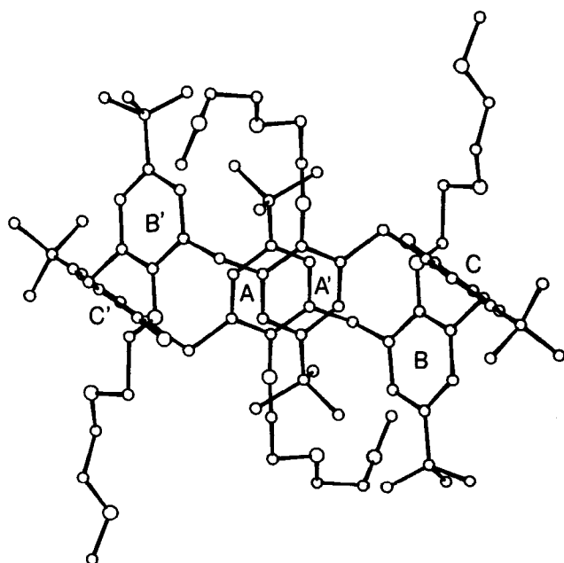
Figure. X-ray structure of compound 11
