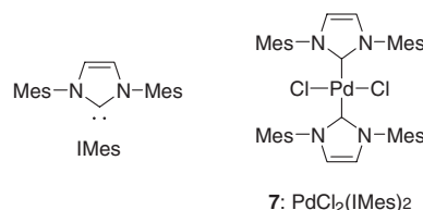
Figure 2. IMes and its Pd complex.
