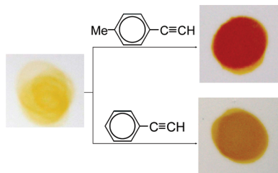
Figure 6. Color changes observed for [\text{PdCl}_2(\text{L}2)] -silica detectors upon exposure to p -tolylacetylene and phenylacetylene.
