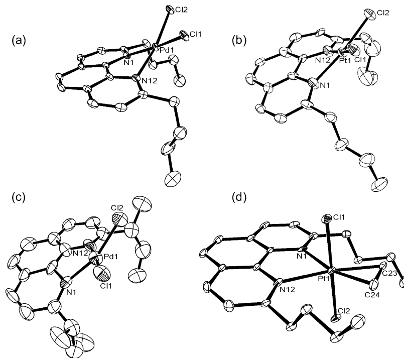
Figure 2. Crystal structures of (a) [\text{PdCl}_2(\text{L}_2)] , (b) [\text{PtCl}_2(\text{L}_2)] , (c) [\text{PdCl}_2(\text{L}_3)] \cdot \text{CHCl}_3 , and (d) [\text{PtCl}_2(\text{C}_2\text{H}_4)(\text{L}_2)] . Hydrogen atoms and solvent molecules have been omitted for clarity. Ortep representations (ellipsoids probability 30%) have been done using Ortep-3 for Windows. 19
