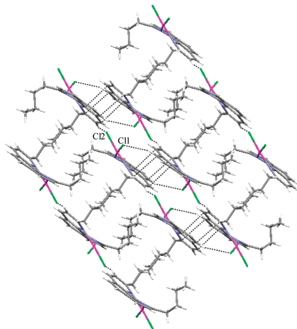
Figure 3. Crystal packing for [\text{PtCl}_2(\text{L2})] showing its layered structure with molecules connected through \pi - \pi (3.22, 3.35 Å) and \text{Cl}\cdots\text{H}-\text{C} interactions (C11...H6A, 2.837 Å; C11-C6, 3.734 Å; C11...H6A-C6, 158°; C12...H3A, 2.815 Å; C12-C3, 3.688 Å; C12...H3A-C3, 152°).
