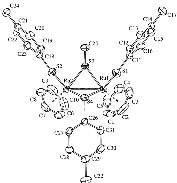
Fig. 1. An ORTEP diagram of (\mu\text{-SMe})(\mu\text{-S-4-C}_6\text{H}_4\text{Me})[\text{CpRu}(\text{S-4-C}_6\text{H}_4\text{Me})_2]_2 ( 5b ). Selected bond lengths (Å) and angles ( ^\circ ) are: \text{Ru}(1)\text{--Ru}(2) = 2.784(10) , \text{Ru}(1)\text{--S}(1) = 2.398(3) , \text{Ru}(1)\text{--S}(3) = 2.319(2) , \text{Ru}(1)\text{--S}(4) = 2.325(2) , \text{Ru}(2)\text{--S}(2) = 2.387(2) , \text{Ru}(2)\text{--S}(3) = 2.332(2) , \text{Ru}(2)\text{--S}(4) = 2.30(2) , \text{Ru}(2)\text{--Ru}(1)\text{--S}(1) = 115.58(6) , \text{Ru}(2)\text{--Ru}(1)\text{--S}(3) = 53.49(5) , \text{Ru}(2)\text{--S}(3)\text{--Ru}(1) = 73.45(6) , \text{S}(1)\text{--Ru}(1)\text{--S}(3) = 93.75(5) , \text{S}(1)\text{--Ru}(1)\text{--S}(4) = 80.08(7) , \text{S}(3)\text{--Ru}(1)\text{--S}(4) = 92.25(7) , \text{Ru}(1)\text{--Ru}(2)\text{--S}(2) = 92.25(7) , \text{Ru}(1)\text{--Ru}(2)\text{--S}(3) = 115.92(6) , \text{Ru}(1)\text{--Ru}(2)\text{--S}(4) = 53.06(5) , \text{S}(2)\text{--Ru}(2)\text{--S}(3) = 53.31(5) , \text{S}(2)\text{--Ru}(2)\text{--S}(4) = 81.80(7) , \text{S}(3)\text{--Ru}(2)\text{--S}(4) = 92.03(7) , \text{Ru}(2)\text{--S}(4)\text{--Ru}(1) = 73.53(7) , \text{S}(3)\text{--Ru}(1)\text{--S}(2) = 92.36(7) .
