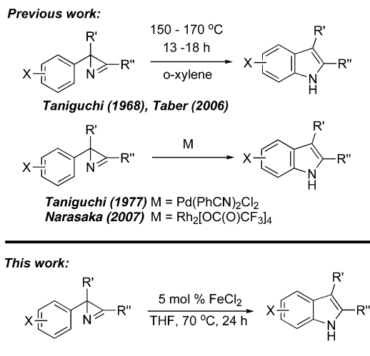
Scheme 1. Rearrangement of 2 H -Azirines to Indoles
