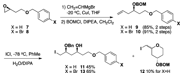
Scheme 2. Synthesis of 1,3- syn Diol Mono Ether 13
