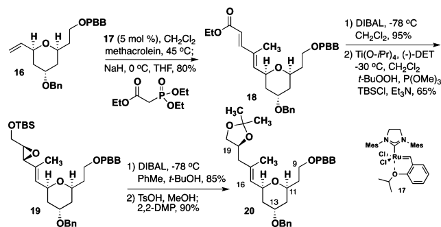
Scheme 4. Completion of C16–C20 Fragment
