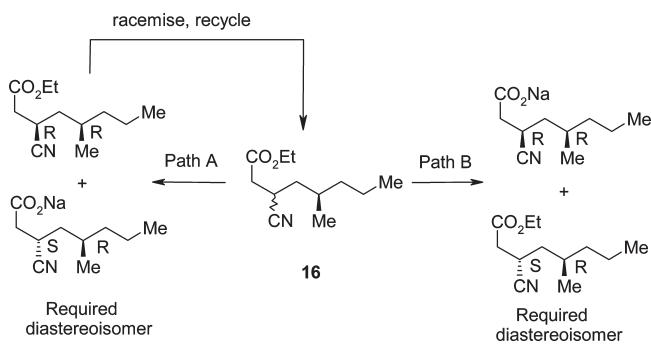
Scheme 5. Enzymatic resolution of ethyl (5 R )-3-cyano-5-methyloctanoate 16
