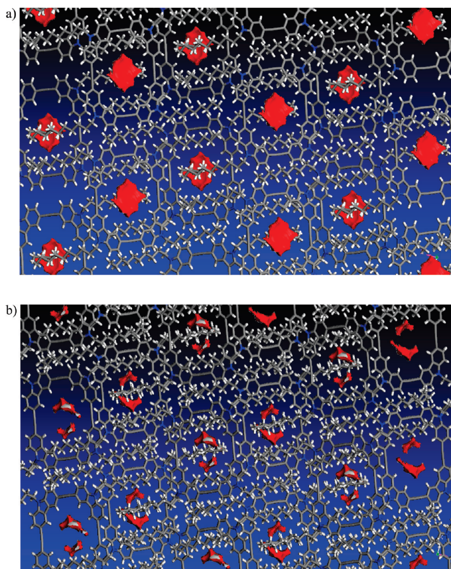
Figure 4. Visualization of the solvent volumes in (a) 2a ·DCM and (b) 2a ·MeOH. Solvent volumes are shown in red. The solvent void area in 2a ·MeOH is significantly smaller than that in 2a ·DCM as a result of the alkyl-chain disorder.
