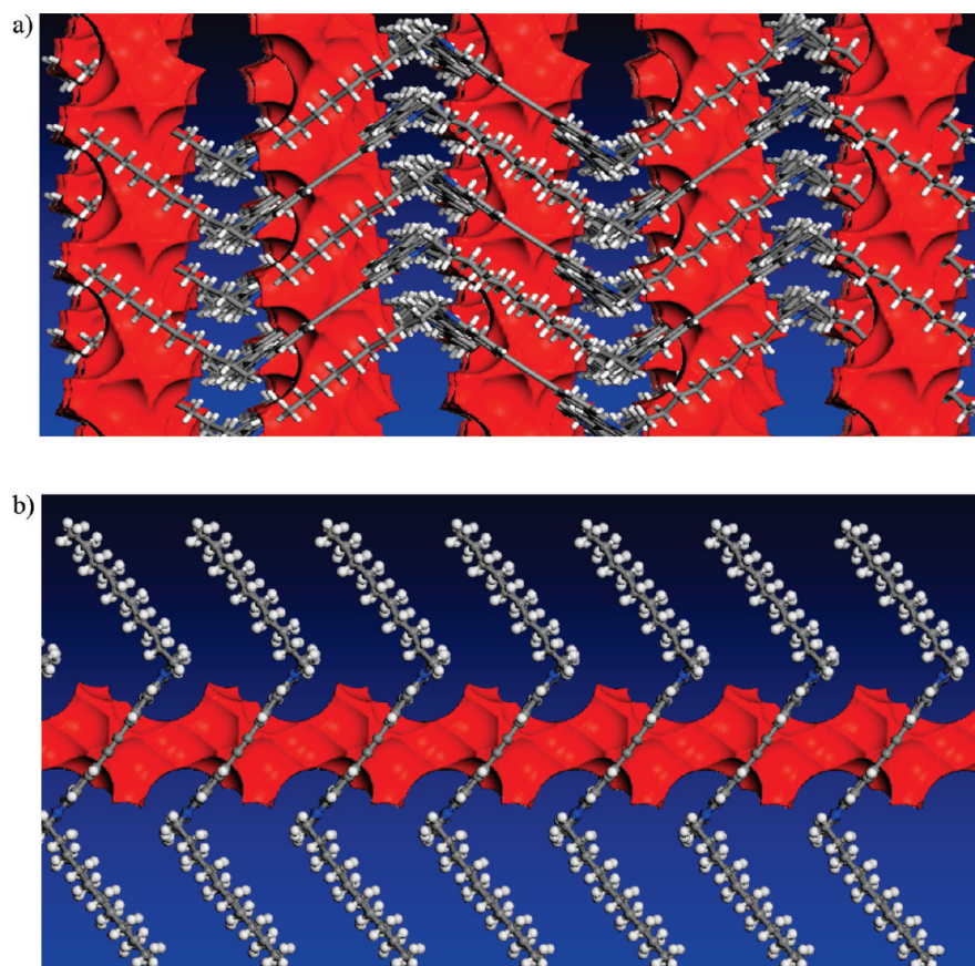
Figure 5. Visualization of the solvent channels in 2b ·DCM viewed down (a) the a axis and (b) the c axis. Solvent channels are shown in red.
