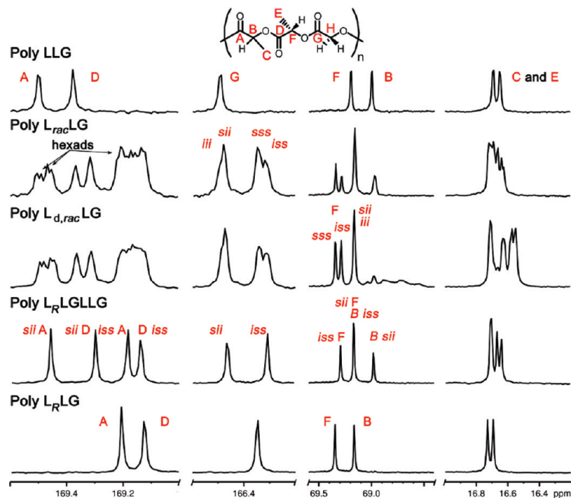
Figure 11. ^{13}\text{C} NMR spectra of L 0 -variable LLG polymers at 175 MHz in \text{CDCl}_3 . Comparisons of the expansions of selected regions for poly LLG , L rac LG , L d, rac LG , L R LGLLG , and L R LG .
