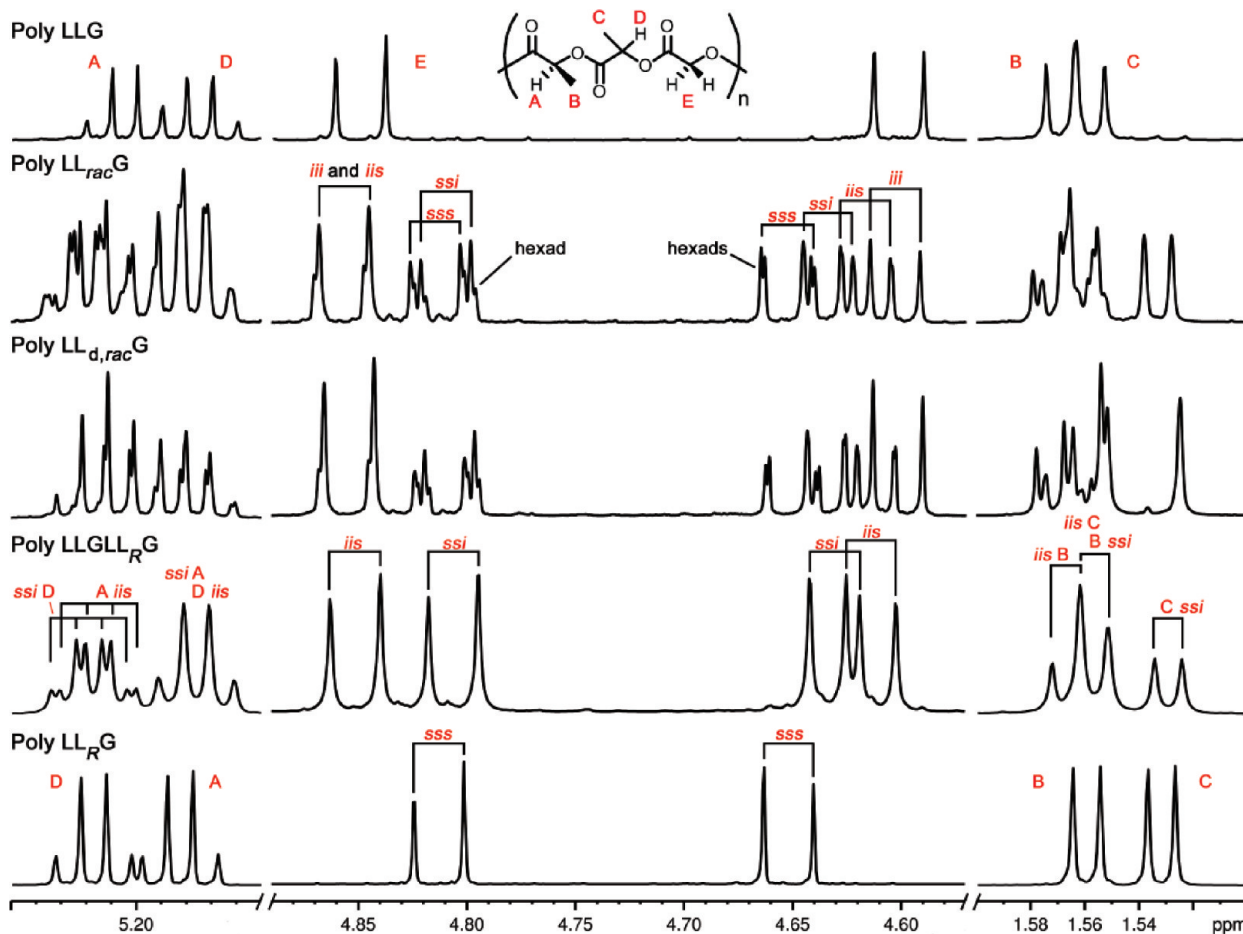
Figure 8. ^1\text{H} NMR spectra of \text{L}^{\text{C}} -variable LLG polymers at 700 MHz in \text{CDCl}_3 . Comparisons of the expansions of selected regions for poly LLG , LL rac G , LL d,rac G , LLGLL R G , and LL R G .
