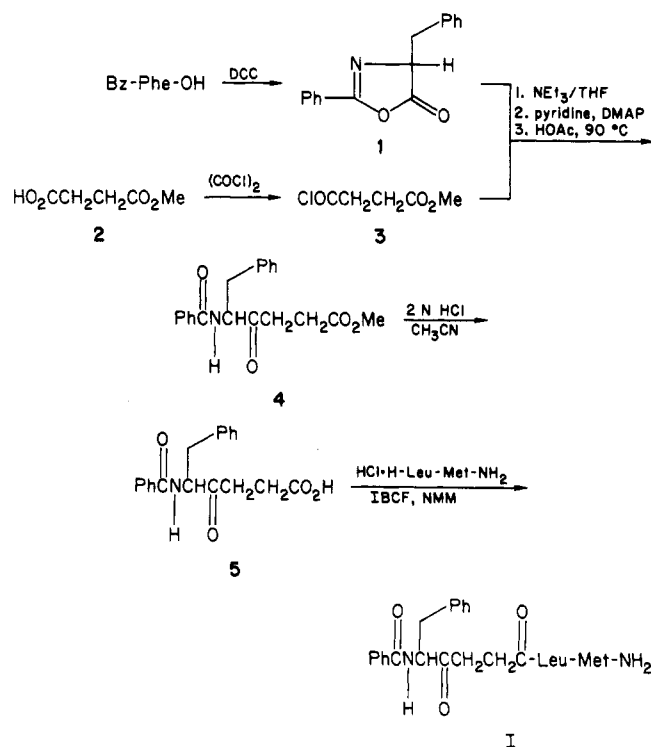
Scheme I
