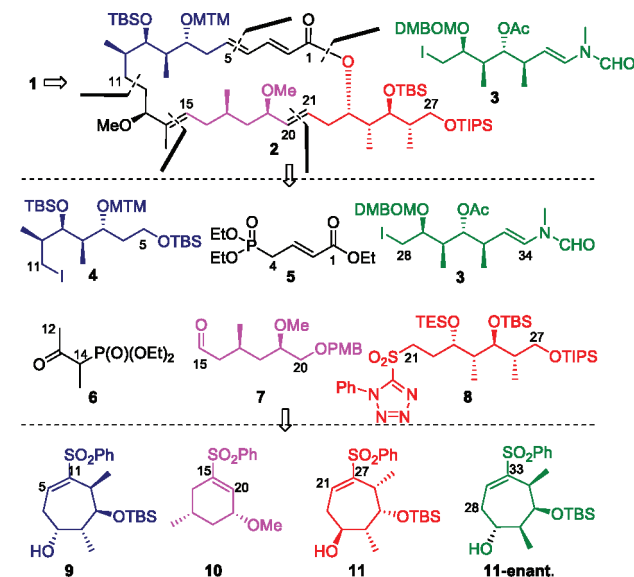
Scheme 1. Retrosynthetic Analysis
