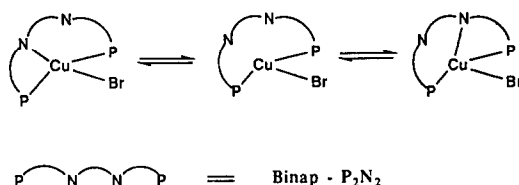
Scheme 1. Proposed mechanism for the dynamic behaviour of II .
