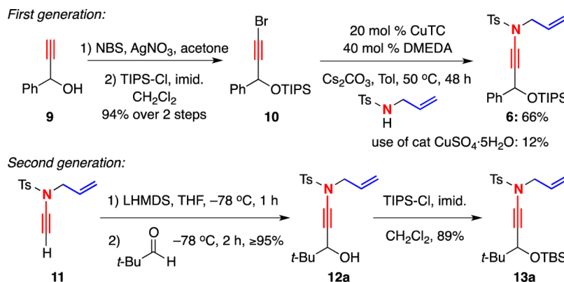
Scheme 3. Preparation of \gamma -Branched Ynamides
