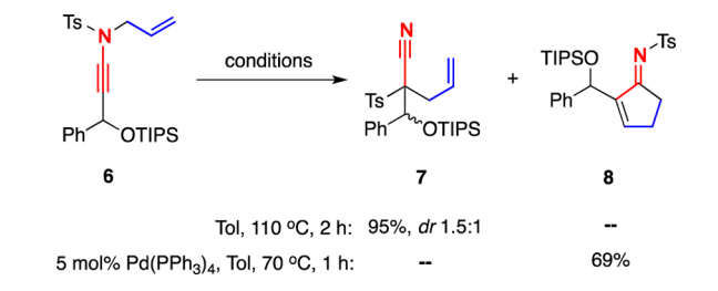
Scheme 2. 1,3-Sulfonyl Shift versus Carbocyclization Dichotomy
