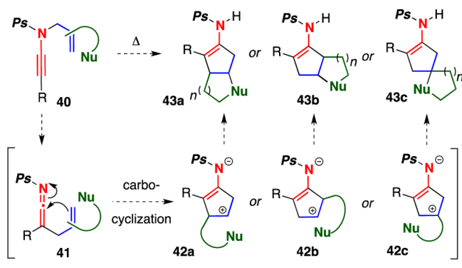
Scheme 8. Potential Carbocyclization Cascades of N -Phosphoryl Ynamides
