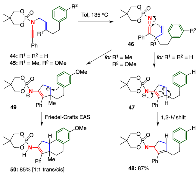
Scheme 9. Carbocyclization Cascade vs 1,2- H Shift
