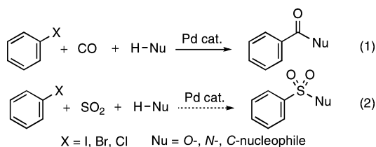
Scheme 1. Palladium-Catalyzed Carbonylation and Sulfonylation Reactions
