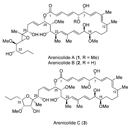
Figure 1. Structures of arenicolides A (1), B (2), and C (3).
