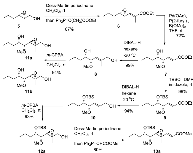
Scheme 2. Synthesis of Intermediate 13a
