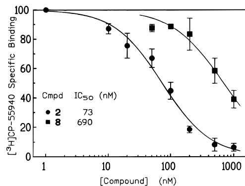
Figure 1. Affinity of 1-naphthyl[2-methyl-1-[2-(4-morpholinyl)ethyl]-1H-indol-3-yl]methanone ( 2 ) (●) and (4-isothiocyanato-1-naphthyl)[2-methyl-1-[2-(4-morpholinyl)ethyl]-1H-indol-3-yl]methanone ( 8 ) (■) for the cannabinoid receptor in brain membranes. [ 3 H]CP-55940 was present at 1.1 nM. Data points are the mean ± standard error from five (compound 2 ) and three (compound 8 ) individual experiments, each performed in triplicate.
