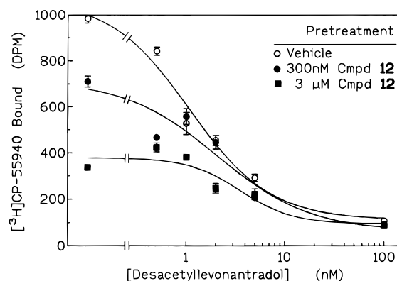
Figure 5. Dose dependency of the covalent binding of isothiocyanate 12 to the cannabinoid receptor. Rat brain membranes were incubated at 30 ^{\circ} C for 60 min with vehicle ( \circ ), or 300 nM ( \bullet ) or 3 \mu M ( \blacksquare ) compound 12 . After sedimentation and resuspension of the membranes, binding of 0.175 nM [ ^3 H]CP-55940 to 50 \mu g of membrane protein was assessed. The data are the mean \pm standard error of the triplicates within a single representative experiment.
