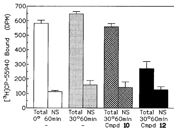
Figure 4. Irreversible decrease in specific binding of [ ^3 H]CP-55940 after pretreatment of rat brain membranes with the isothiocyanate 12 but not 10 . Pretreatment of membranes with either 1 \mu M 12 (solid) or 10 (hatched) was performed at 30 ^{\circ} C for 60 min. Controls included parallel incubations of membranes with vehicle (0.05% \beta -cyclodextrin plus 0.01% dimethyl sulfoxide) at either 30 ^{\circ} C (stipled) or 0 ^{\circ} C (open). After washing away of the compounds by sedimentation, cannabinoid receptor binding was quantitated. Data bars are the mean \pm standard error of the total binding and the nonspecific binding (not displaced by 0.1 \mu M desacetyllevonantradol) from three individual experiments, each performed in triplicate.
