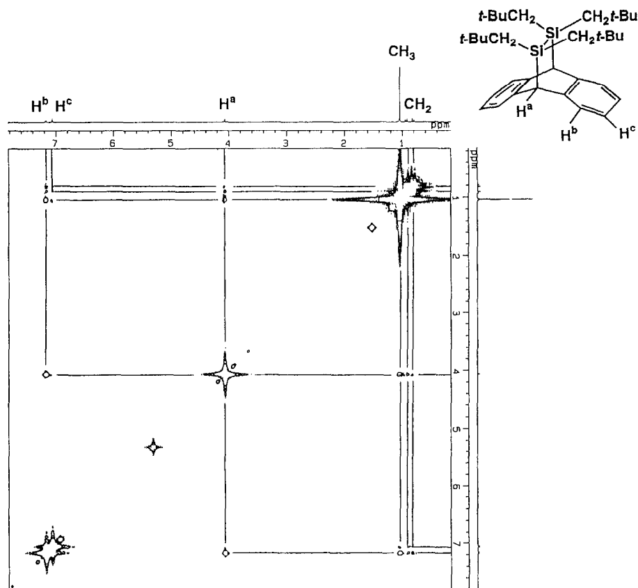
Fig. 2. NOESY spectrum of 1 in CD 2 Cl 2 .
