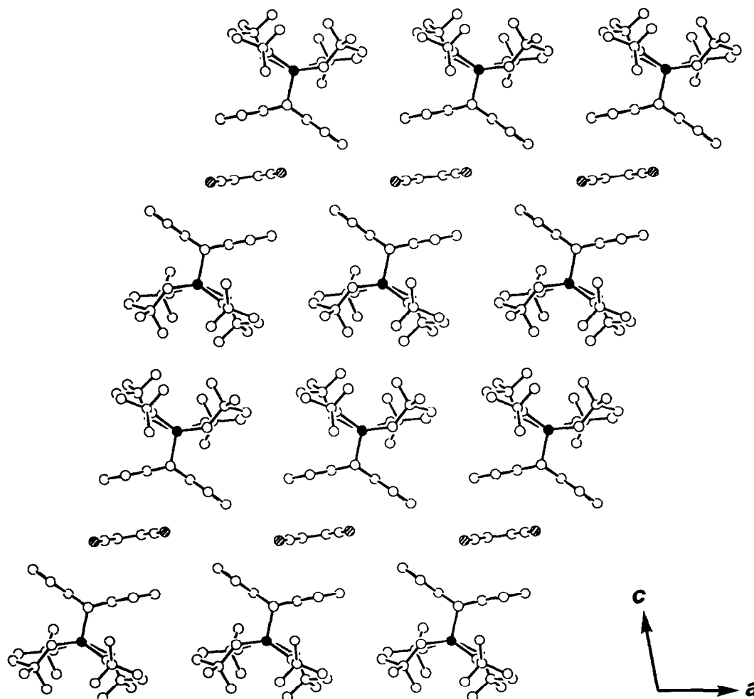
Fig. 6. Packing diagram of the charge-transfer complex of 1 and TCNE viewed along the b axis. The filled circles denote silicon atoms, nitrogen atoms are shaded.
