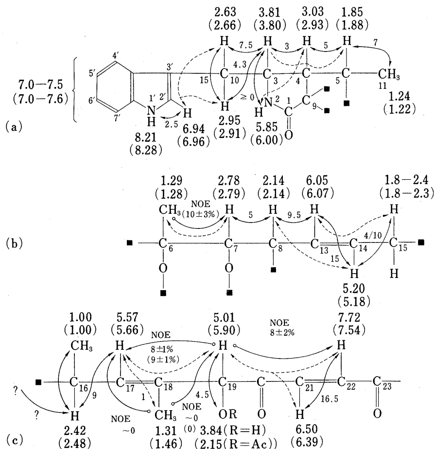
Chart 1. The Partial Structures (a), (b) and (c) and ^1\text{H} -NMR Parameters of Chaetoglobosin A ( \text{R}=\text{H} ) and the Acetate ( \text{R}=\text{Ac} ) (in \text{CDCl}_3 )
