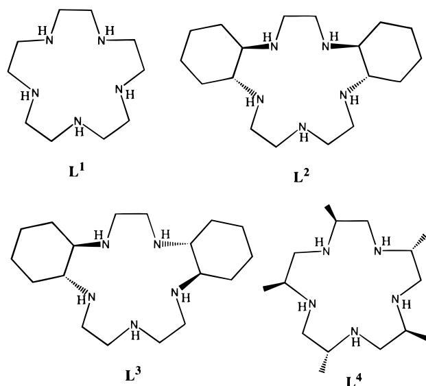
Figure 1. Structures of the pentaaza macrocyclic ligands utilized for the synthesis of \text{Fe}(\text{III}) complexes.
