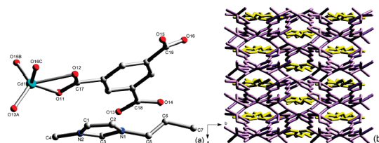
Figure 2. Structure of 3 : (a) asymmetric unit; (b) 3D view with the PMI (yellow) lying in the channels.
