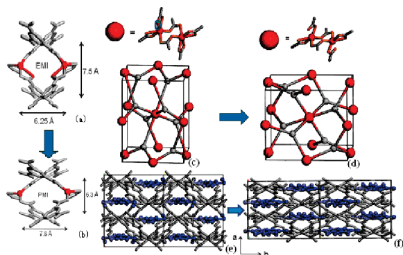
Figure 3. (a and b) Environments of channels occupied with \text{EMI}^+ and \text{PMI}^+ in 2 and 3 , respectively. Note that one \text{Cd}-\text{O} bond (red) is broken on moving from 2 to 3 . (c and d) Topologies of the [\text{Cd}(\text{BTC})]^- networks in 2 and 3 , in which red and gray circles represent \text{Cd}_2 dimers and \text{BTC}^{3-} ligands, respectively. (e and f) Views along [001] directions in compounds 2 and 3 .
