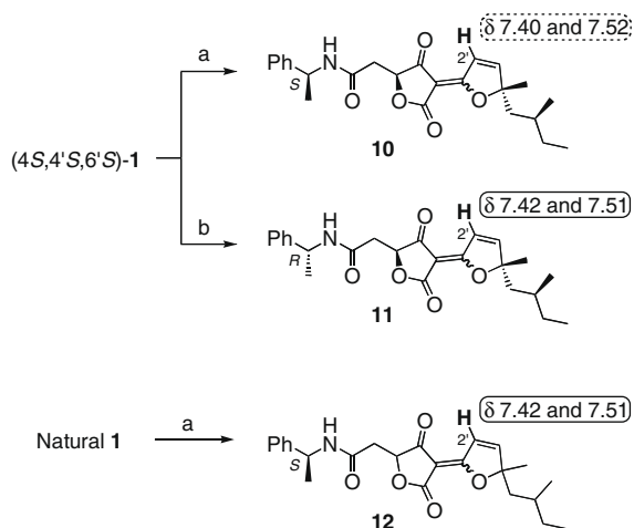
Scheme 5. Determination of the absolute configuration of nodulisporacid A ( 1 ) by 1 H NMR data comparison of (S)- or (R)-1-phenylethylamine derivative. Reagents and conditions: (a) (S)-1-phenylethylamine, EDCI, Et 3 N, CH 2 Cl 2 ; (b) (R)-1-phenylethylamine, EDCI, Et 3 N, CH 2 Cl 2 .
