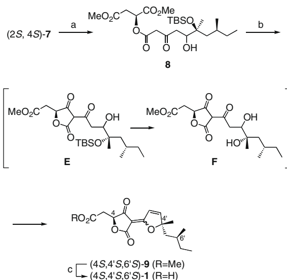
Scheme 3. Synthesis of (4 S ,4' S ,6' S )- 1 . Reagents and conditions: (a) diketene (2 equiv), TiCl 4 (1.2 equiv), CH 2 Cl 2 , −78 °C, 15 min then dimethyl ( S )-malate (2 equiv), −78 to 0 °C, over 3 h, 62%; (b) TBAF (1 equiv), THF, 0 °C to rt, 1 h, then TBAF (2 equiv), rt, 20 h, then concd HCl, rt, 5 h, 51%; (c) 6 N HCl, 1,4-dioxane, rt, 97%.
