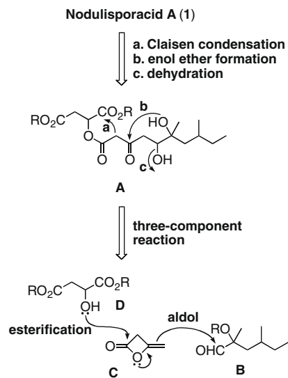
Scheme 1. Retrosynthetic analysis.
