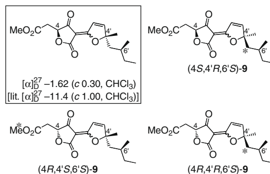
Figure 2. Synthesized stereoisomers of nodulisporacid A methyl ester.
