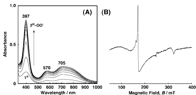
Figure 2. (A) Spectral changes during the reaction of 1 H (0.2 mM) and O 2 in 9:1 acetone–CH 3 CN at −85 °C. (B) X-band fine-structure ESR spectrum of 2 H –OO • observed in the microwave parallel-excitation mode ( B 0 // B 1 ) in 9:1 acetone–CH 3 CN at 3 K. The microwave frequency used was 9.37007 GHz. The forbidden half-field transitions observed at g ≈ 4 in the conventional perpendicular mode appear as allowed ones with strong intensities.
