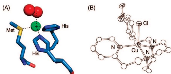
Figure 1. (A) Structure of the Cu B active center of oxy-PHM. 11 (B) Crystal structure of 2 NO 2 –Cl, with thermal ellipsoids showing 50% probability. The counteranion and the hydrogen atoms have been omitted for clarity.
