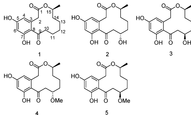
FIGURE 1. Curvarin (1), 11- \alpha -hydroxycurvarin (2), 11- \beta -hydroxycurvarin (3), 11- \alpha -methoxycurvarin (4), and 11- \beta -methoxycurvarin (5).
