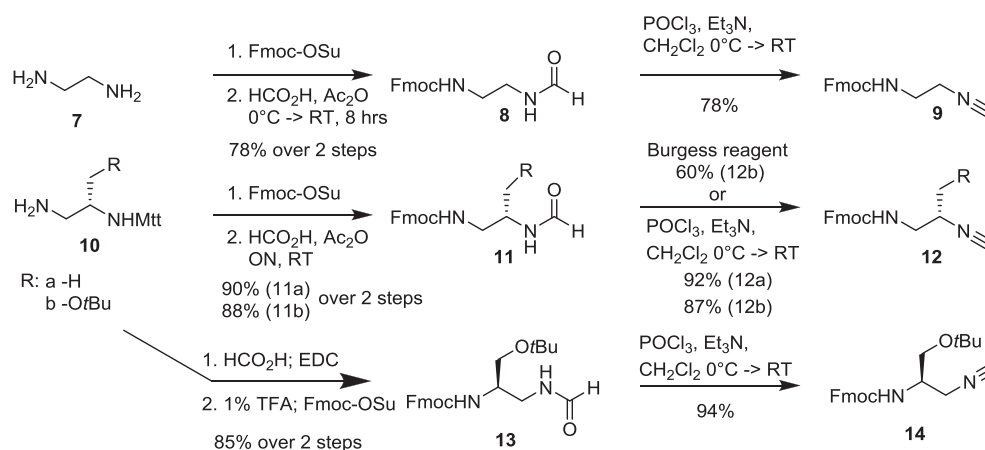
Fig. 3. Synthesis of isocyanide 9–14.
