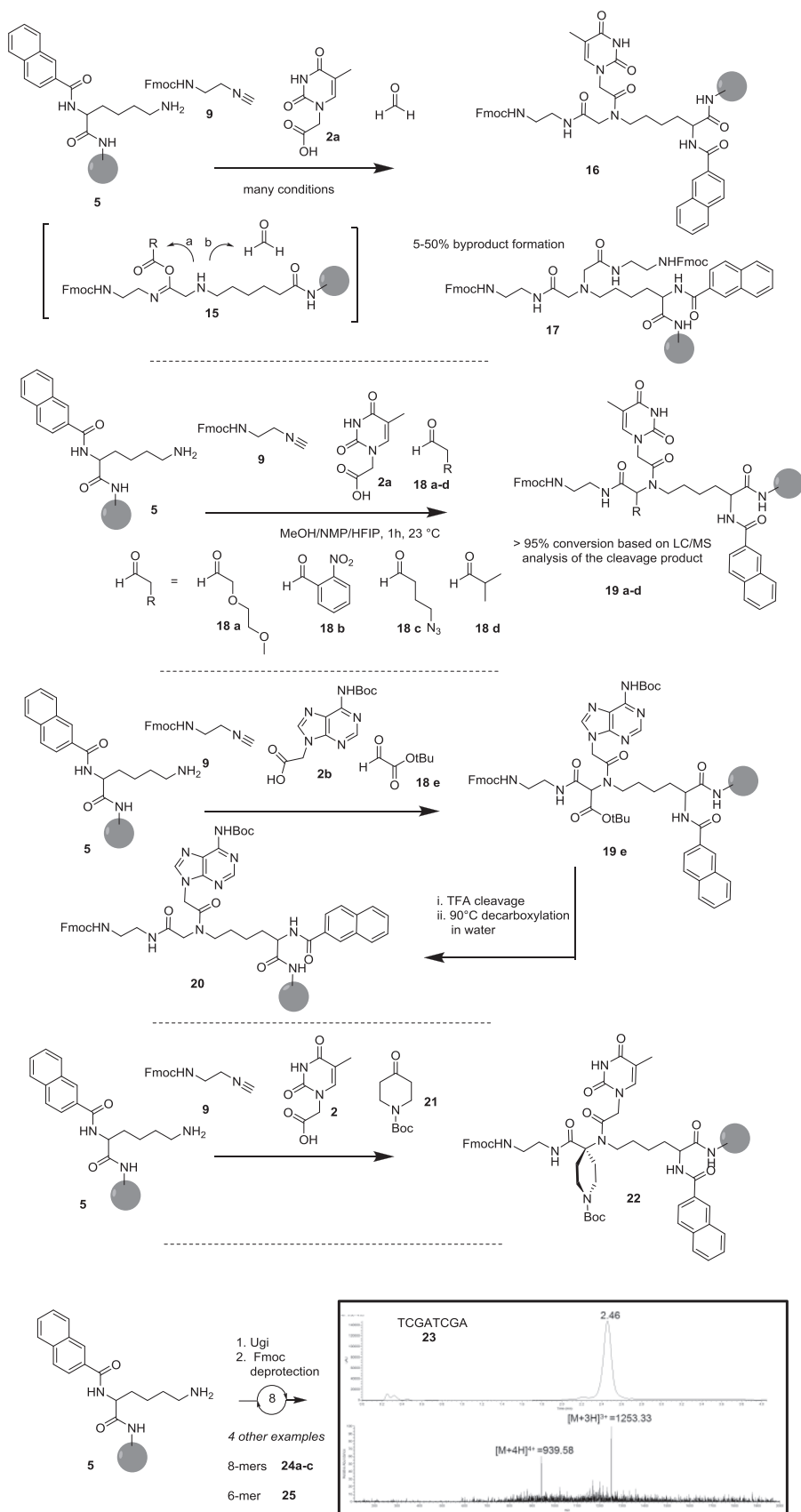
Fig.4. Ugi oligomerization in the N to C direction, method 2.
