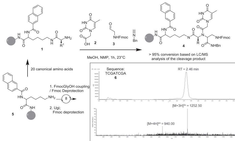
Fig. 2. PNA synthesis by C to N Ugi couplings, method 1.
