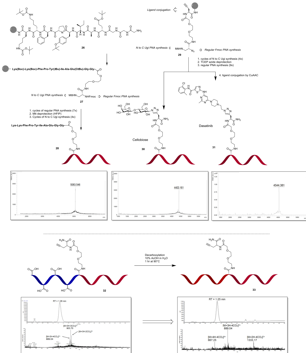
Fig. 5. Application of bi-directional synthesis for the preparation of PNA-ligand conjugates at defined position in the oligomer backbone Decarboxylation of a bi-directional PNA 8-mer.
