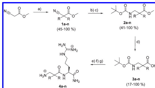
Scheme 1. Overview of Synthesis of the \beta -Peptidomimetics 4a–n a
