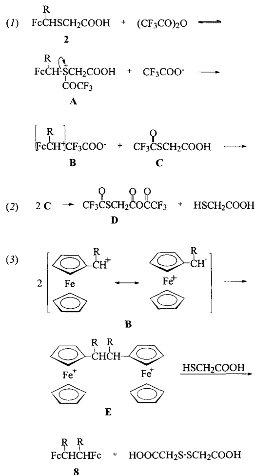
Scheme 3.
