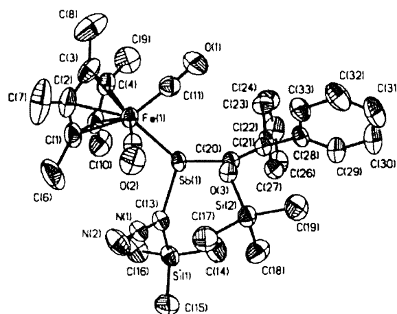
Fig. 2. Molecular structure of 4c in the crystal.
