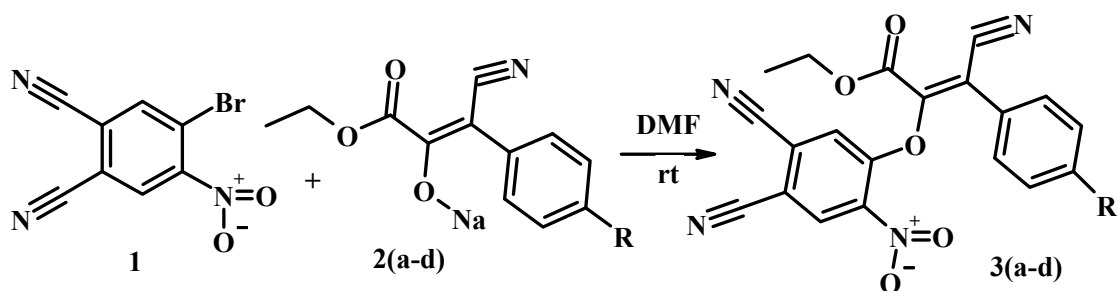
Scheme 1. Synthesis of compounds 3(a-d)
