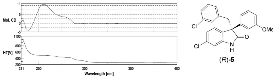
Fig. 3. CD Spectrum of ( R )- 5 ( c = 0.0001\text{M} , in \text{CH}_2\text{Cl}_2 )
