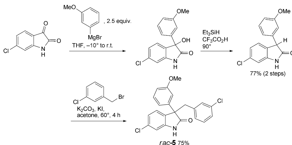
Scheme 2. F. Hoffmann–LaRoche Synthesis of rac-5 [3]
