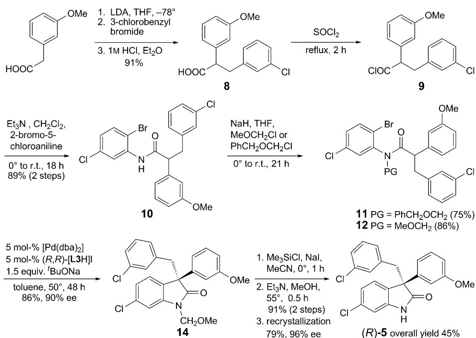
Scheme 4. Catalytic Enantioselective Synthesis of ( R )- 5
