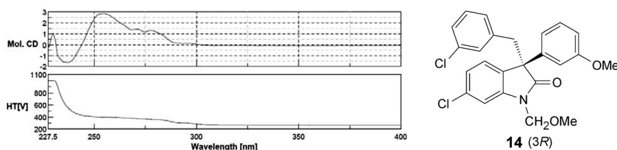
Fig. 2. CD Spectrum of 14 ( c = 0.0001\text{M} , in \text{CH}_2\text{Cl}_2 )
